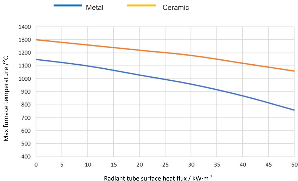
Chart 1 Radiant heat flux vs. furnace temperature
