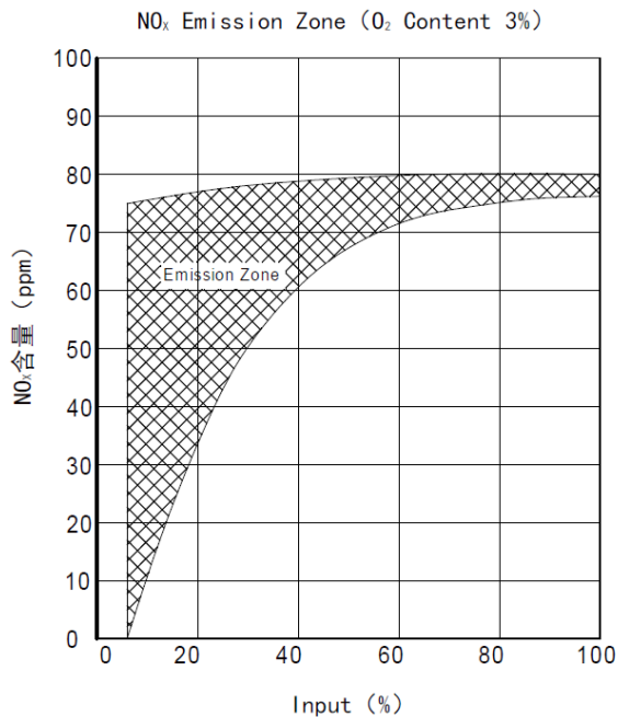
Fig. 4 VFS82G Series Burner NO x Emission Zone
