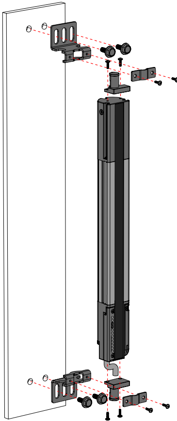
Figure 16. End-Mount Brackets
