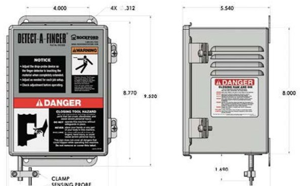
Right Side Mount Control Box (Part No. RKC009)
